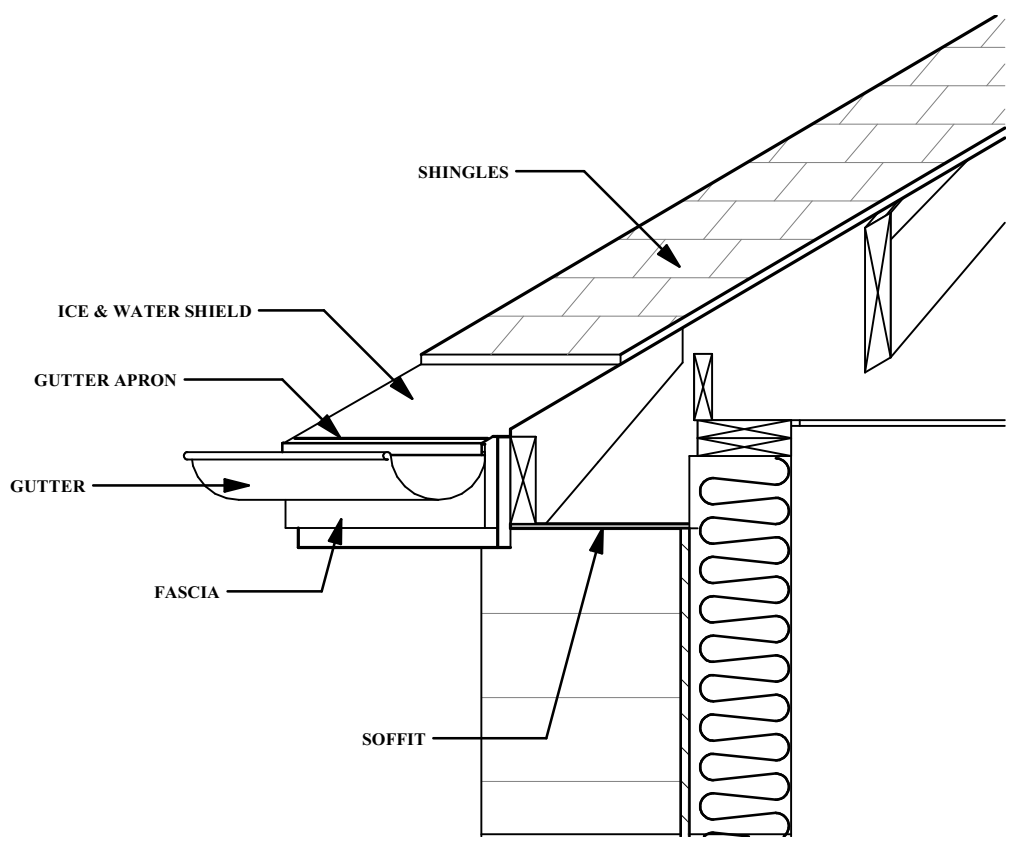
TYPICAL EAVE
